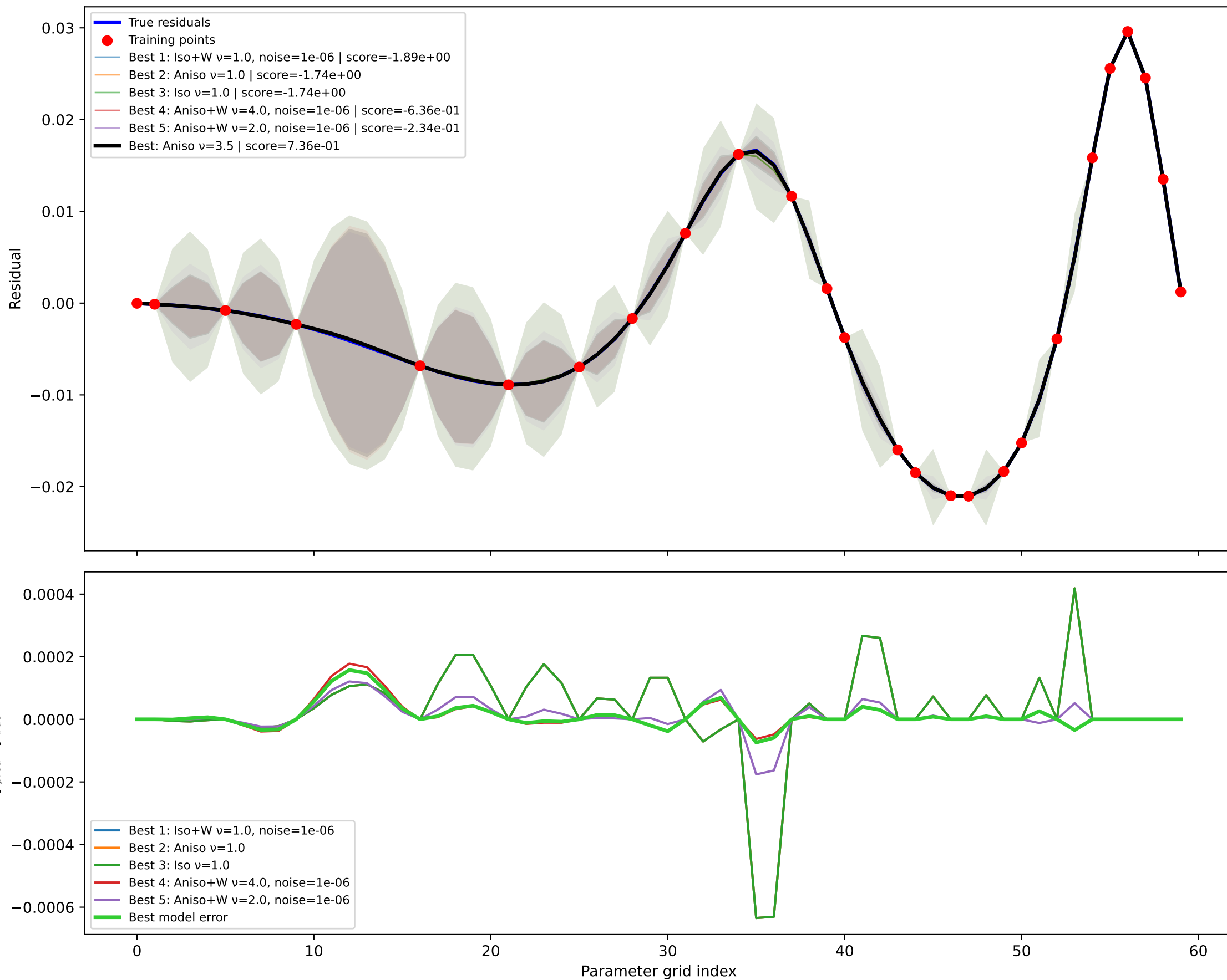
GPR kernel comparison node=25 RMSE=4.179e-05, train RMSE=1.571e-11
